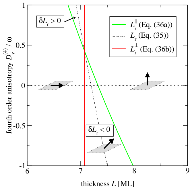
Figure 2: Phase diagram of a fcc Ni-like system in the D_v^{(4)} - L plane. The parameters are 9,20 J/\omega = 10^4 , D_v^{(2)}/\omega = 31 , D_s^{(2)}/\omega = -180 , and D_i^{(2)} = D_{s,i}^{(4)} = 0 .
