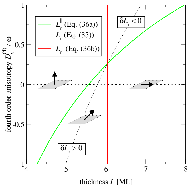
Figure 1: Phase diagram of a sc Fe-like system in the D_v^{(4)} - L plane. The parameters are 9,20 J/\omega = 2.6 \times 10^3 , D_s^{(2)}/\omega = 37 , and D_{v,i}^{(2)} = D_{s,i}^{(4)} = 0 .
