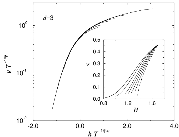
FIG. 3: Scaling plot of the interface velocity for d = 3 . The data are rescaled according to Eq. (6). The inset shows the unscaled velocities for T = 0.025n with n \in \{1, 2, 3, 4, 6, 8\} (solid lines) in comparison to the T = 0 data from Fig. 2 (dashed line).
