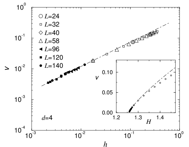
FIG. 4: The interface velocity of the four-dimensional model at T = 0 . For sufficiently small fields the data obey a power law according to Eq. (1) (dotted-dashed line). For the fit we use only those data marked by filled symbols and we find H_c = 1.258 \pm 0.05 and \beta = 0.8 \pm 0.06 .
