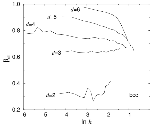
FIG. 6: The effective exponents \beta_{\text{eff}} as a function of \ln h for various dimensions. The figure shows that the five-dimensional exponent does not display a clear saturation as the exponent of the lower dimensions do. The data of the six-dimensional model indicate that the expected saturation value \beta_{\text{eff}} = 1 is reached significantly faster as compared to d = 5 (see text). The values of the two-dimensional system are obtained from [13].
