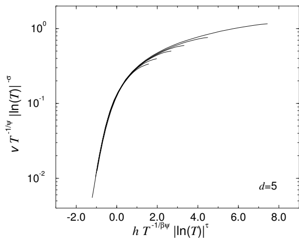
FIG. 8: The scaling plot of the interface velocity v for the five dimensional model, i.e. at the upper critical dimension. The data are rescaled according to Eqs. (10,11) using \psi = 1.49 , \beta = 1 , \sigma = 0.22 , and \tau = 0.19 .
