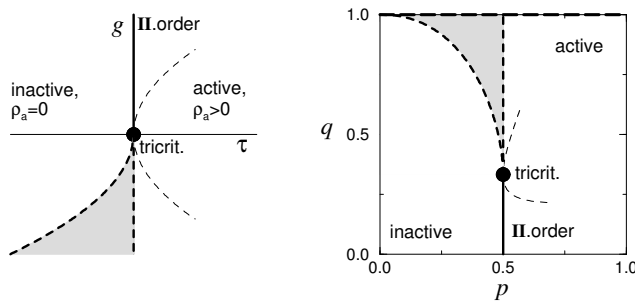
FIG. 1: The mean field phase diagrams of tricritical directed percolation (TDP). The left figure sketches the phase diagram as a function of the coarse grained variables \tau and g [see Eq. (1)]. The right figure shows the corresponding phase diagram as a function of the microscopic variables p and q , as defined by a reaction scheme of the tricritical contact process (see text). The thick lines correspond to second-order phase transitions (II.order) with \beta_{\text{DP}} = 1 . The bold circles mark the transition point of TDP with \beta_t = 1/2 . The shadowed areas indicate the coexistence of the absorbing and the active phase. The thin dashed lines illustrate the crossover to the tricritical behavior. In the right figure, two absorbing phases appear for q = 1 (long dashed lines). These phases are the fully occupied lattice (stable for q > 0 ) and the empty lattice (stable for q < 1/2 ).
