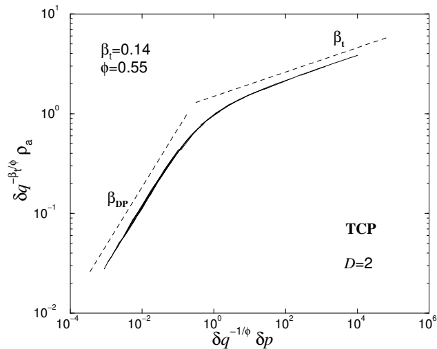
FIG. 4: The crossover scaling function of the order parameter at zero field. The dashed lines correspond to the asymptotic behaviors, i.e., to the ordinary DP and to the tricritical DP behavior [see Eq. (30)].
