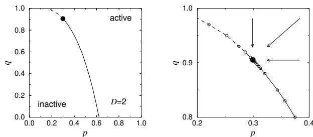
FIG. 7: The phase diagram of the two-dimensional modified contact process. The solid line marks continuous phase transitions which belong to the universality class of directed percolation. The dashed line corresponds to first-order phase transitions and the bold circle indicates the tricritical point. The small circles in the right figure show where the transitions points are determined numerically. Furthermore, the tricritical point is approached in the simulations along three different ways illustrated by the three arrows.
