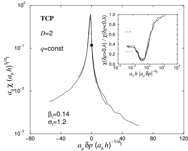
FIG. 12: The universal scaling function \tilde{\chi}(x, 0, 1) of the universality class of tricritical directed percolation. The circle marks the condition \tilde{\chi}(0, 1, 0) = \beta_t / \sigma_t and reflects the accuracy of the performed analysis. The inset displays the universal ratio \tilde{\chi}(1, 0, x) / \tilde{\chi}(-1, 0, x) . The extrapolation ( x \rightarrow 0 ) yields the value of the universal amplitude ratio \tilde{\chi}(1, 0, 0) / \tilde{\chi}(-1, 0, 0) = 0.35 \pm 0.04 . The obtained value differs significantly from the corresponding values (dashed lines) of ordinary directed percolation 0.25 for D = 2 and 0.65 for D = 3 [35], respectively.
