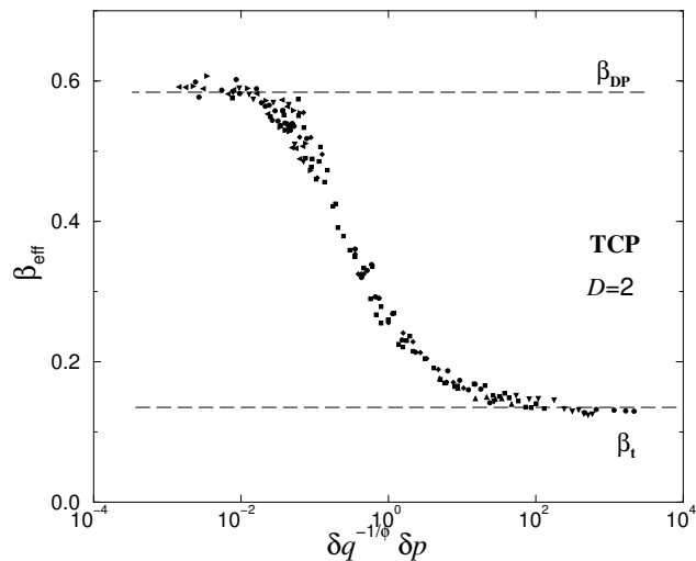
FIG. 5: The effective exponent \beta_{\text{eff}} of the order parameter. Both asymptotic scaling regimes ( \beta_t and \beta_{DP} ) as well as the crossover regime are clearly recovered.
